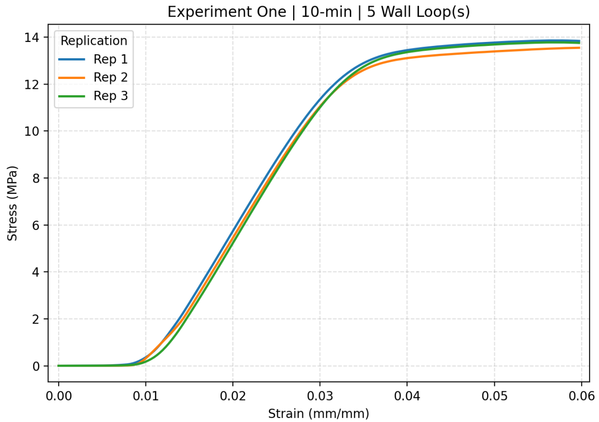
Figure C.6. The stress strain curve of Experiment one 10-min with 5 wall loops including all replications.
