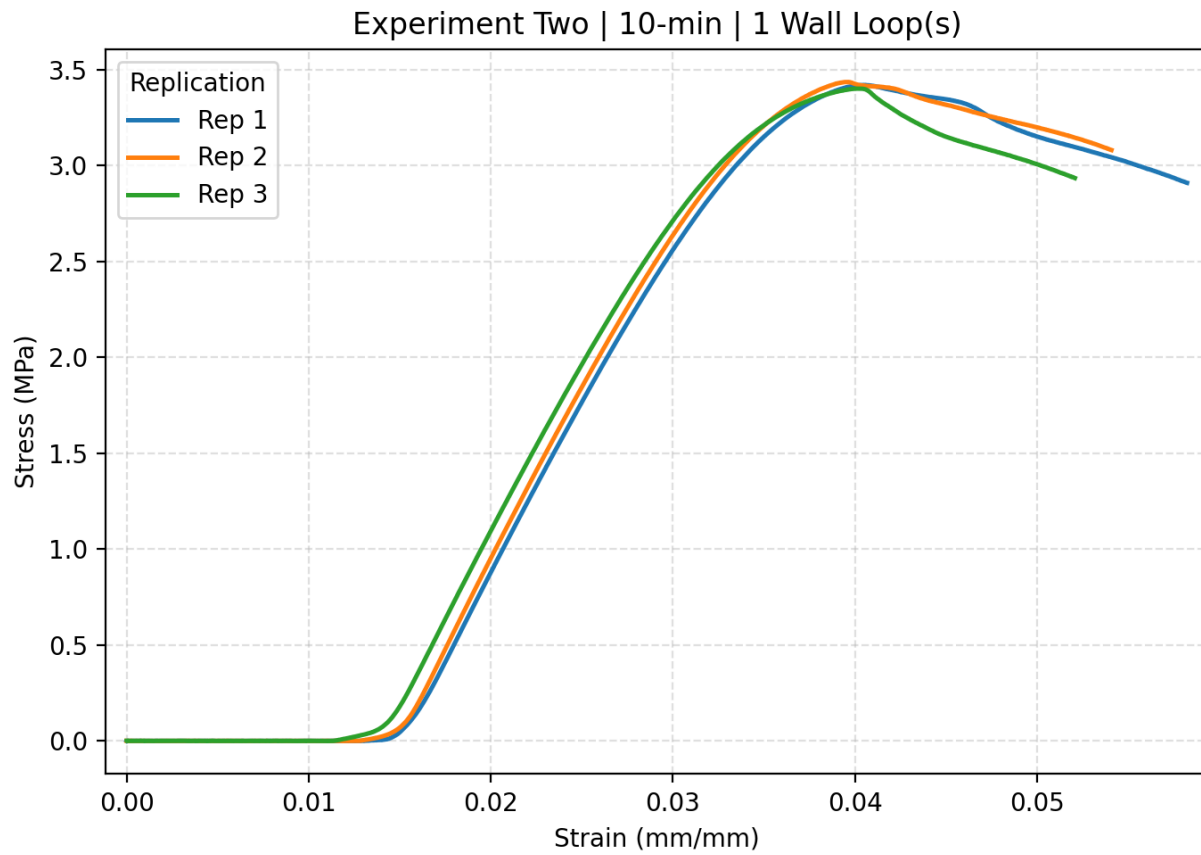
Figure C.16. The stress strain curve of Experiment two 10-min with 1 wall loop including all replications.
