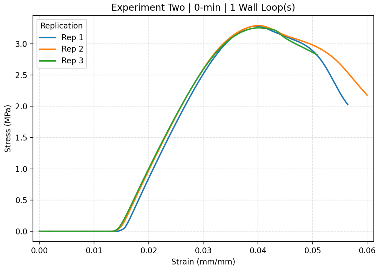
Figure C.13. The stress strain curve of Experiment two 0-min with 1 wall loop including all replications.
