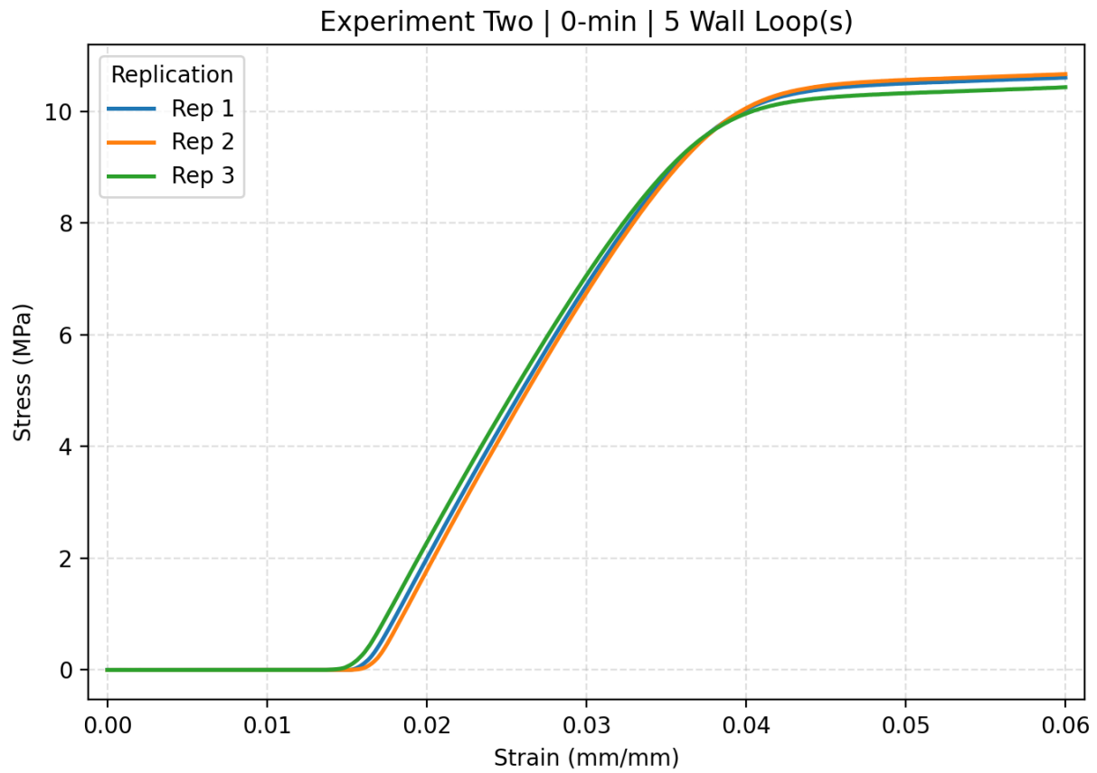
Figure C.15. The stress strain curve of Experiment two 0-min with 5 wall loops including all replications.
