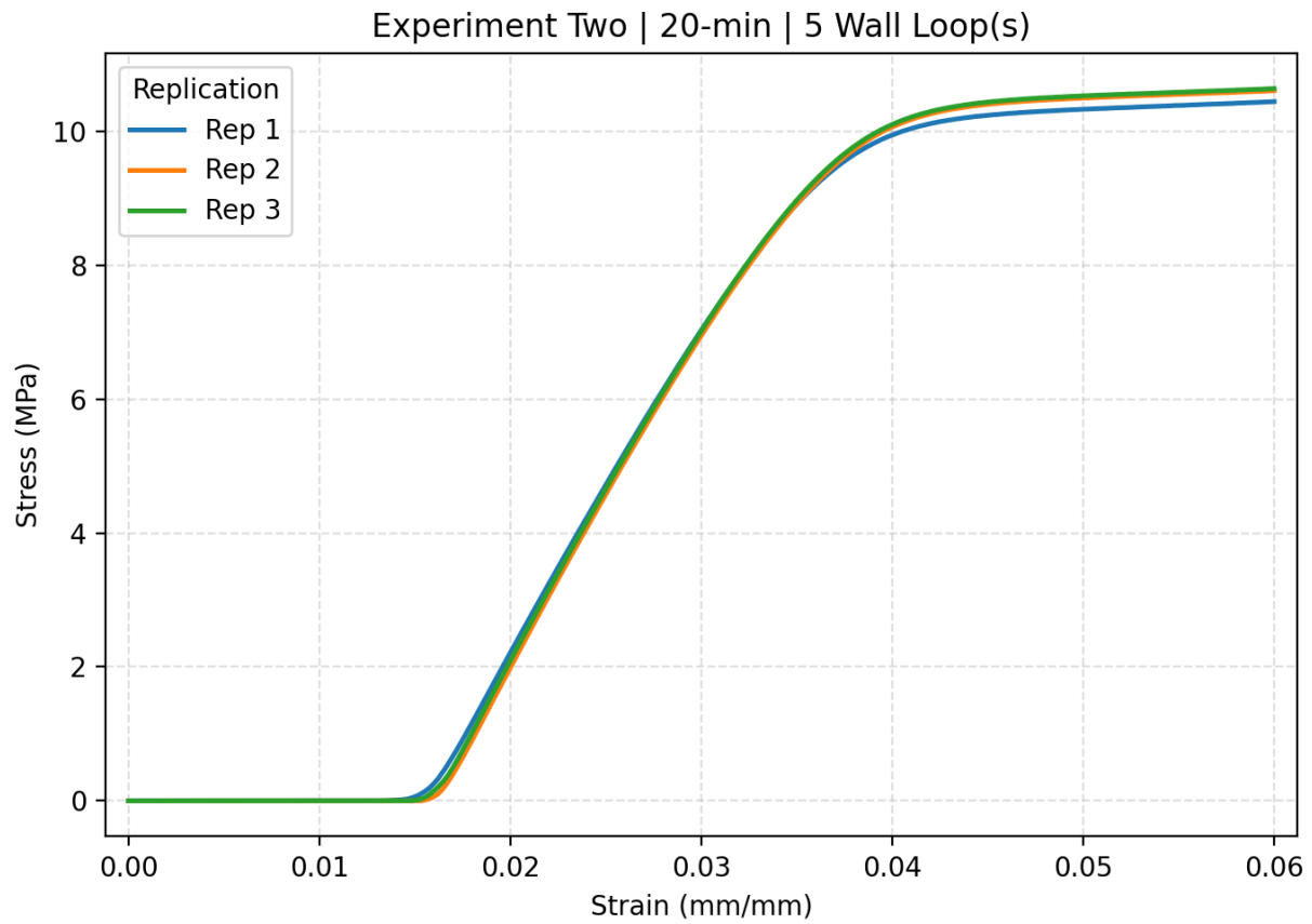
Figure C.21. The stress strain curve of Experiment two 20-min with 5 wall loops including all replications.
