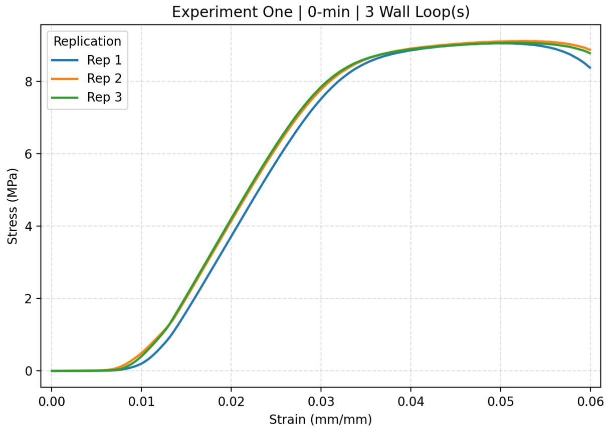
Figure C.2. The stress strain curve of Experiment one 0-min with 3 wall loops including all replications.
