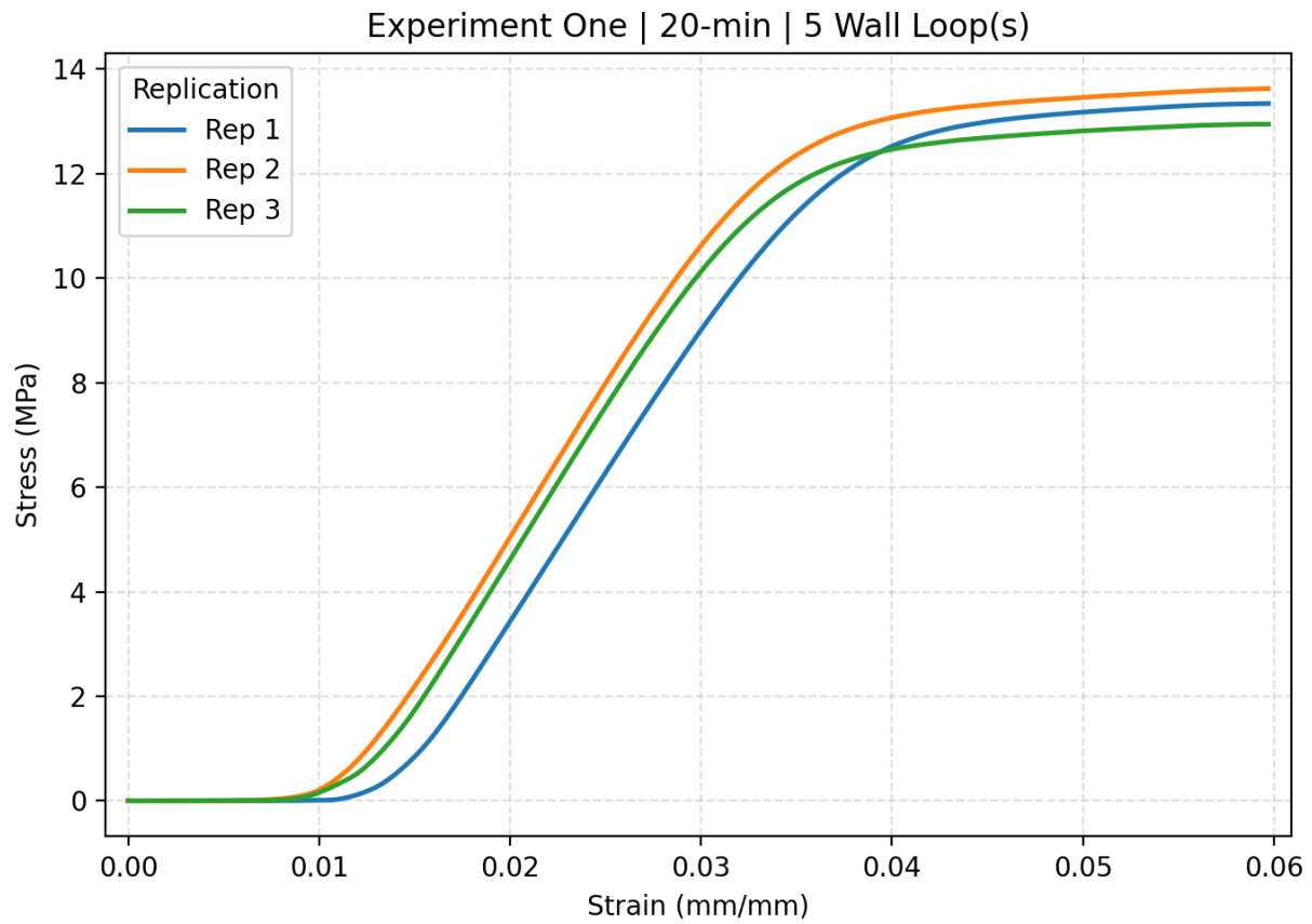
Figure C.9. The stress strain curve of Experiment one 20-min with 5 wall loops including all replications.
