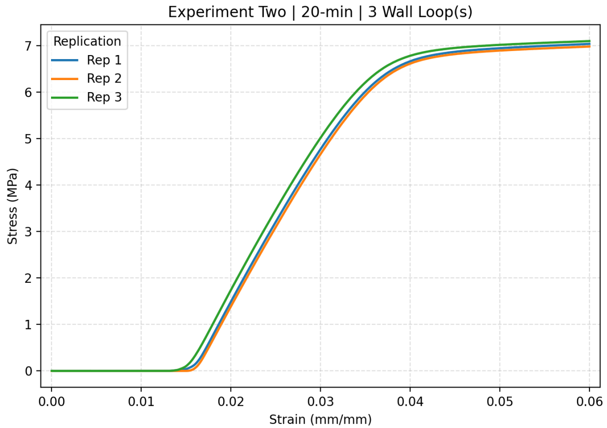
Figure C.20. The stress strain curve of Experiment two 20-min with 3 wall loops including all replications.
