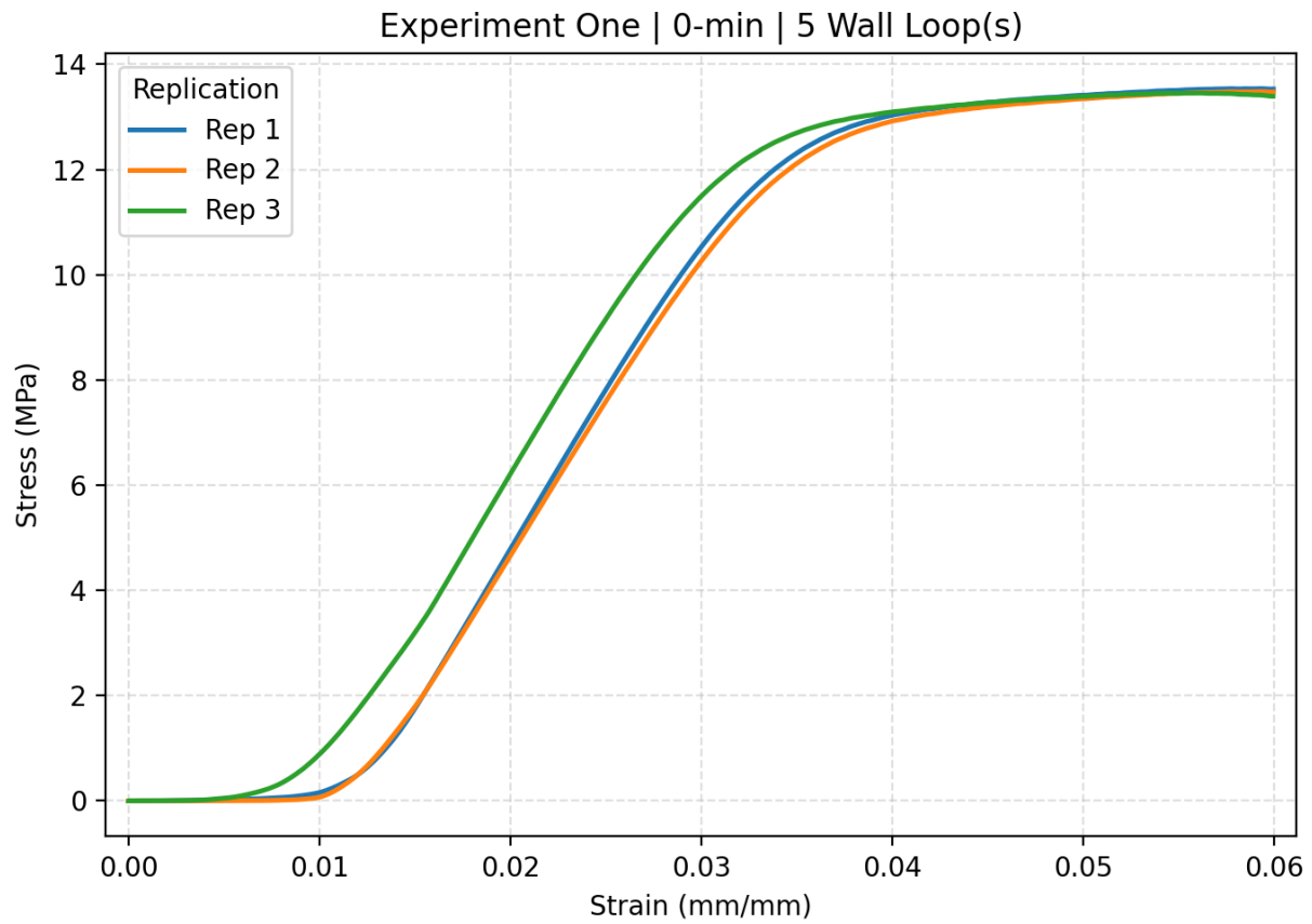
Figure C.3. The stress strain curve of Experiment one 0-min with 5 wall loops including all replications.
