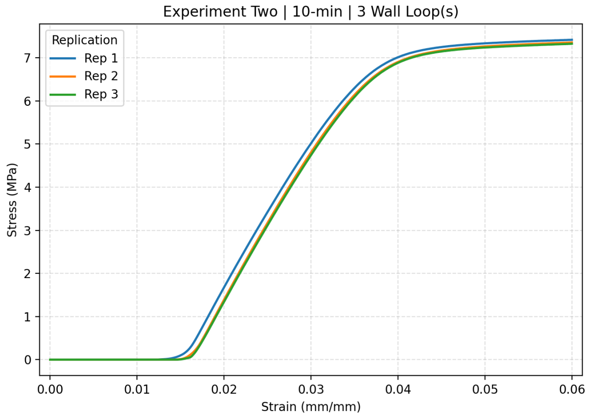
Figure C.17. The stress strain curve of Experiment two 10-min with 3 wall loops including all replications.
