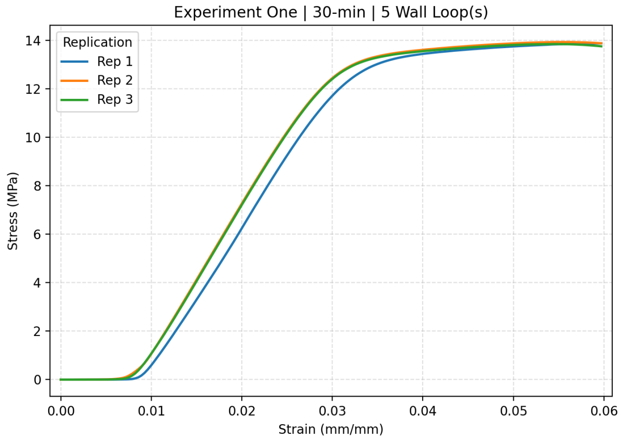
Figure C.12. The stress strain curve of Experiment one 30-min with 5 wall loops including all replications.
