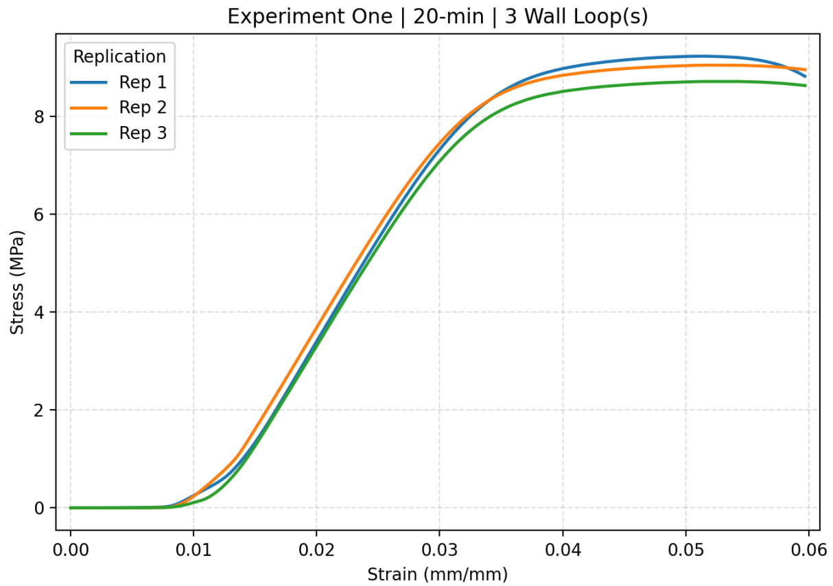
Figure C.8. The stress strain curve of Experiment one 20-min with 3 wall loops including all replications.
