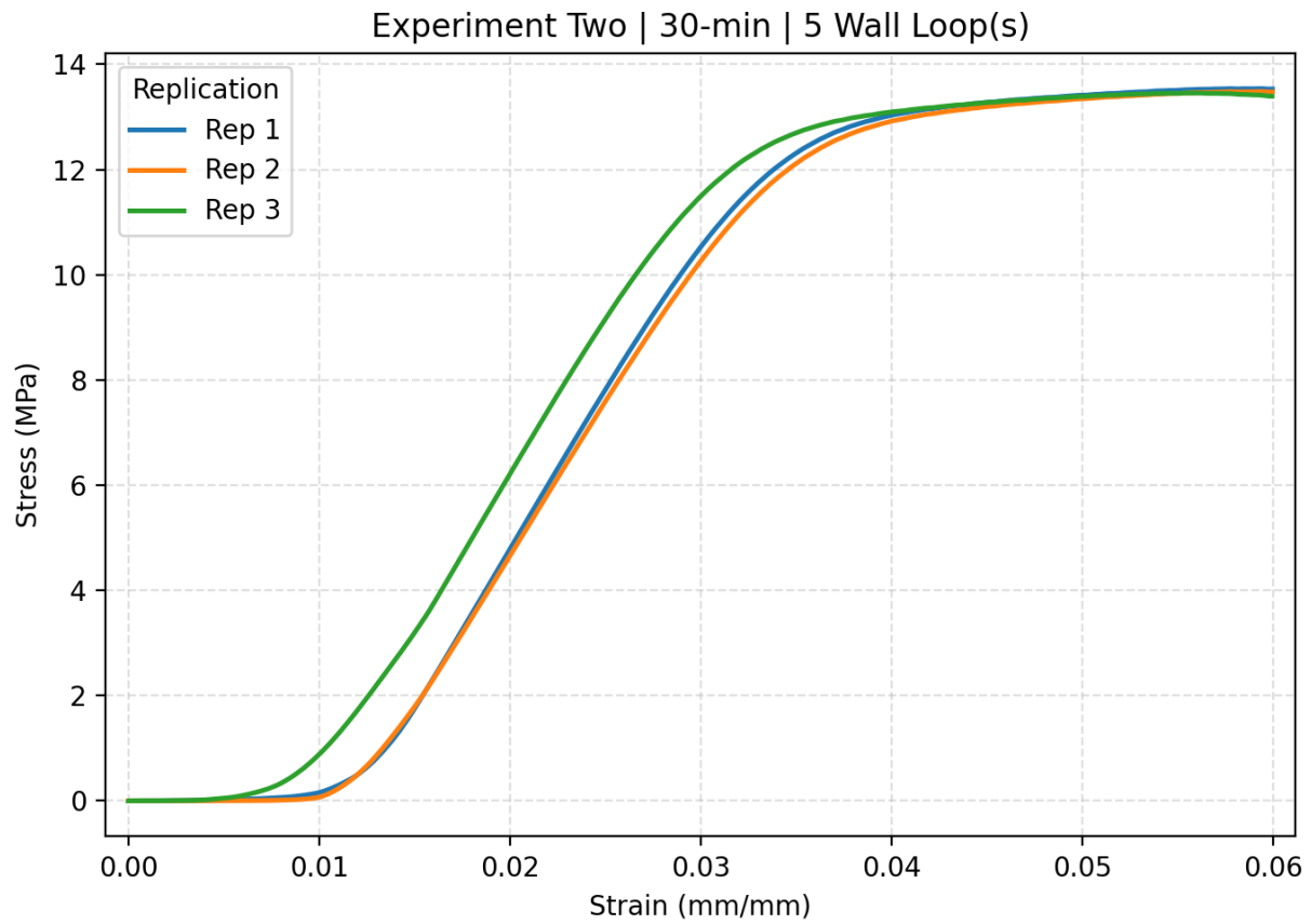
Figure C.24. The stress strain curve of Experiment two 30-min with 5 wall loops including all replications.
