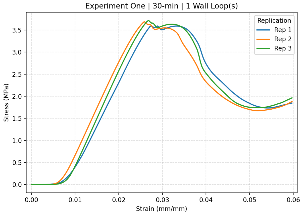
Figure C.10. The stress strain curve of Experiment one 30-min with 1 wall loop including all replications.
