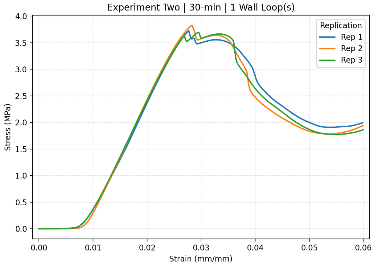
Figure C.22. The stress strain curve of Experiment two 30-min with 1 wall loop including all replications.
