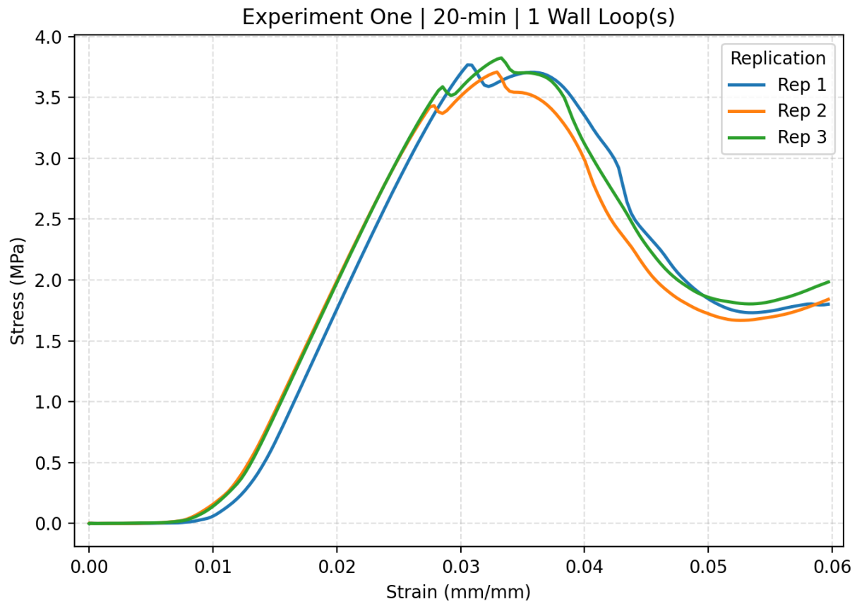
Figure C.7. The stress strain curve of Experiment one 20-min with 1 wall loop including all replications.
