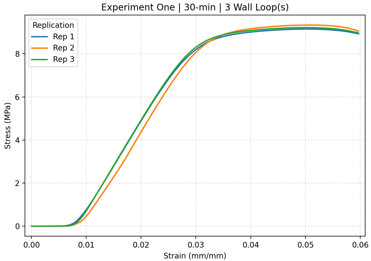
Figure C.11. The stress strain curve of Experiment one 30-min with 3 wall loops including all replications.
