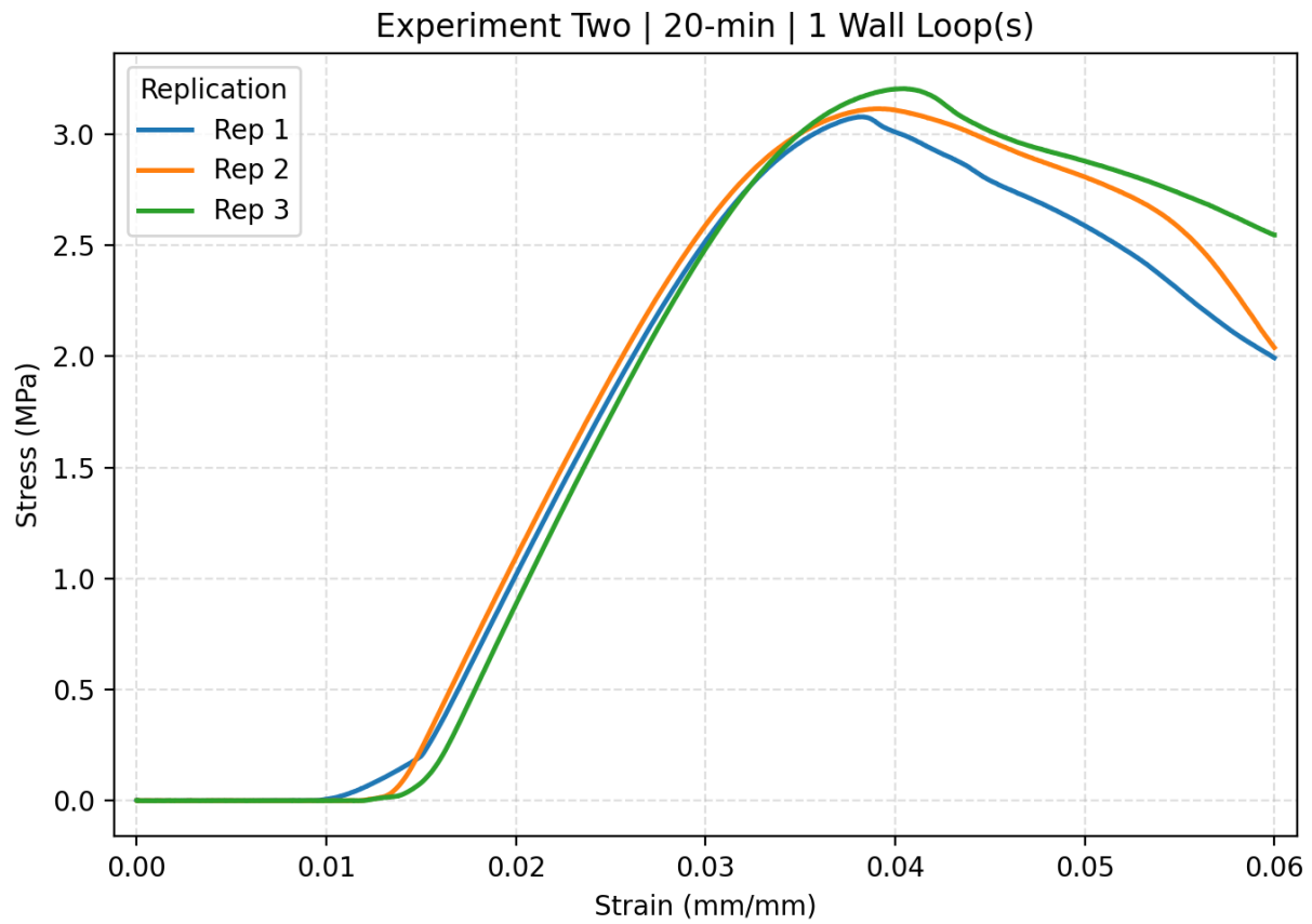
Figure C.19. The stress strain curve of Experiment two 20-min with 1 wall loop including all replications.
