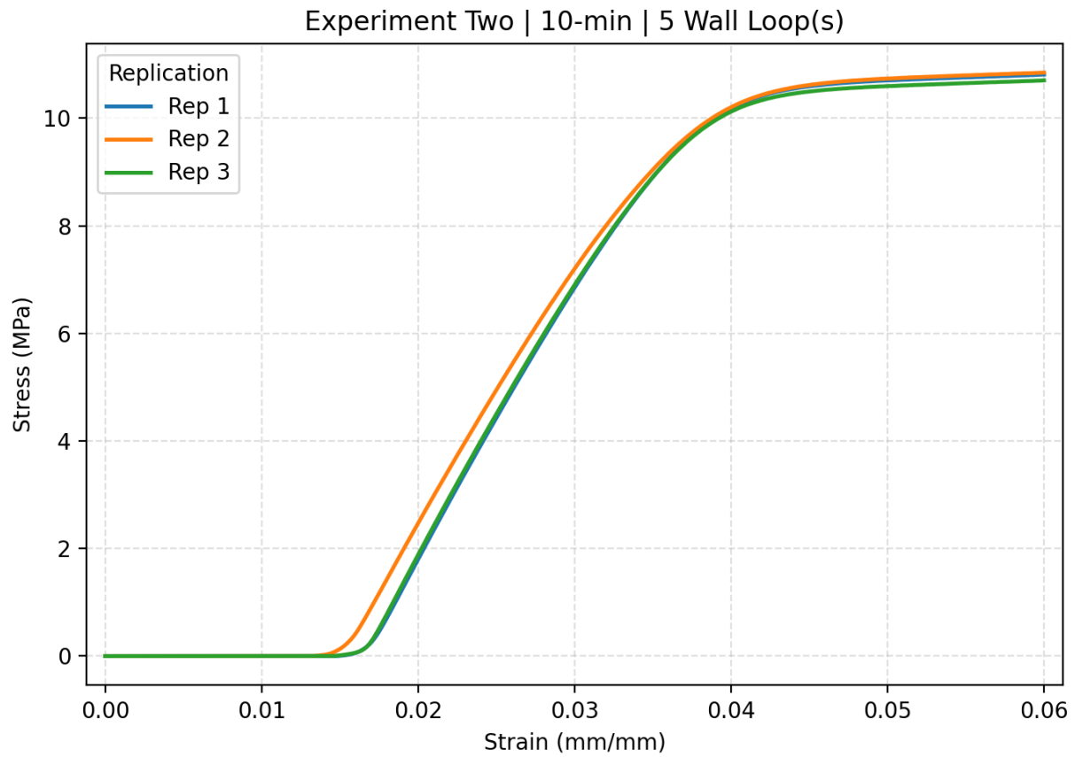
Figure C.18. The stress strain curve of Experiment two 10-min with 5 wall loops including all replications.
