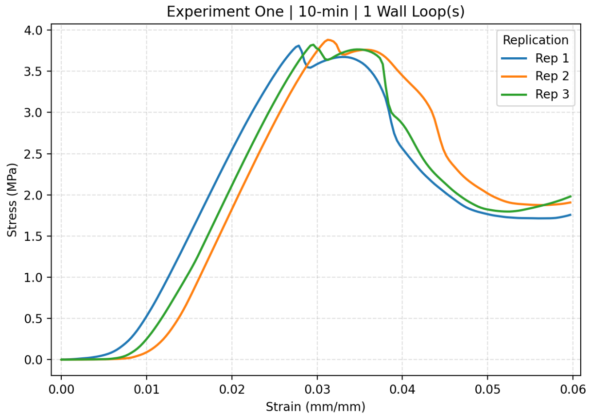
Figure C.4. The stress strain curve of Experiment one 10-min with 1 wall loop including all replications.
