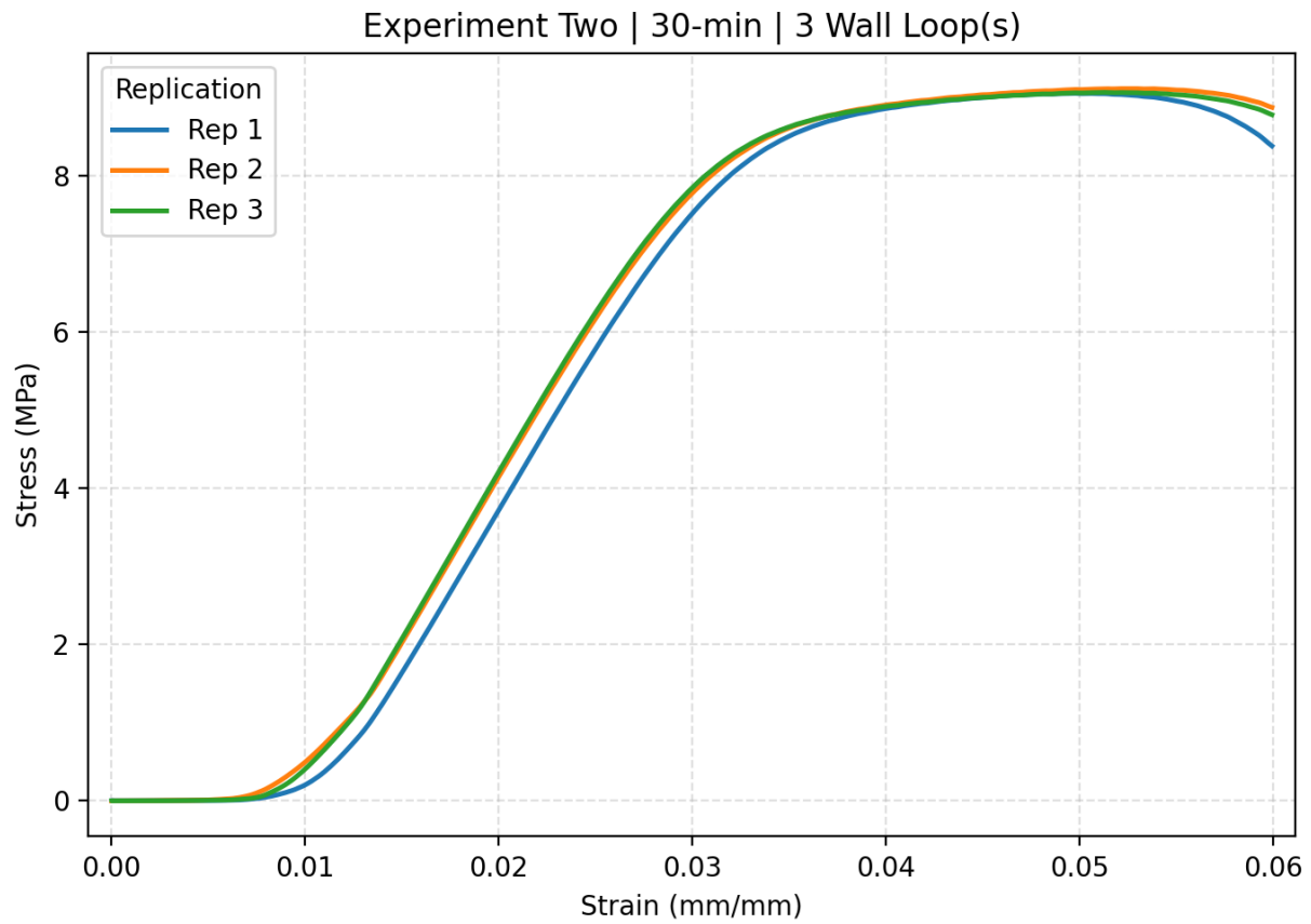
Figure C.23. The stress strain curve of Experiment two 30-min with 3 wall loops including all replications.
