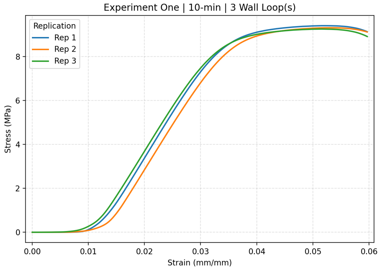
Figure C.5. The stress strain curve of Experiment one 10-min with 3 wall loops including all replications.
