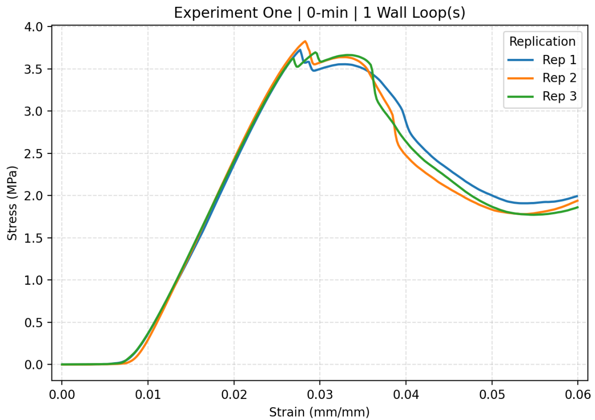
Figure C.1. The stress strain curve of Experiment one 0-min with 1 wall loop including all replications.
