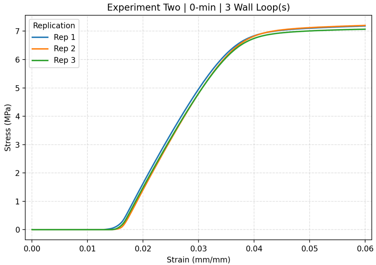
Figure C.14. The stress strain curve of Experiment two 0-min with 3 wall loops including all replications.
